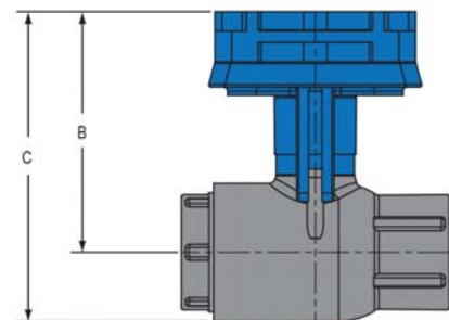
Compact 2000 Ball Valve (66-Series)
