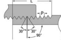
AMERICAN NATIONAL STANDARD TAPER PIPE THREADS (NPT) ANSI B1 .20.1 ASTM F 1498
